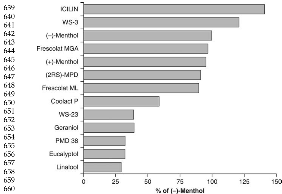
Figure 11 Efficacy of coolants on the TRPM8 receptor (by Ca 2+ fluorometric assay). Source: From Refs. 72, 73, 88.
