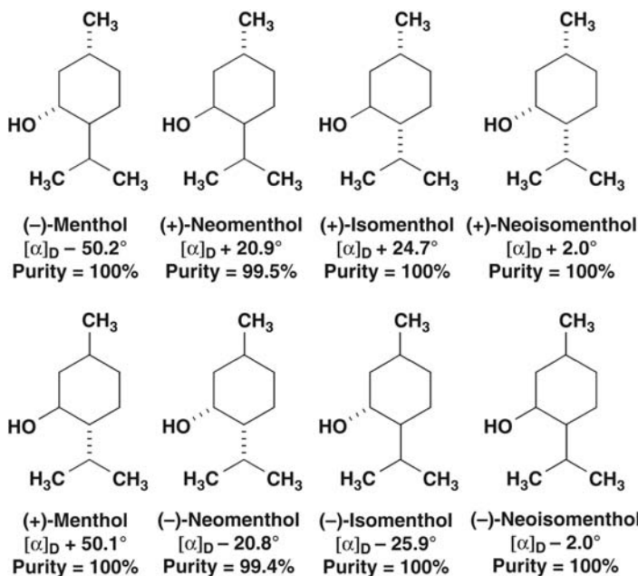
Figure 1 Stereoisomers of menthol. Source: From Ref. 14. Q10
